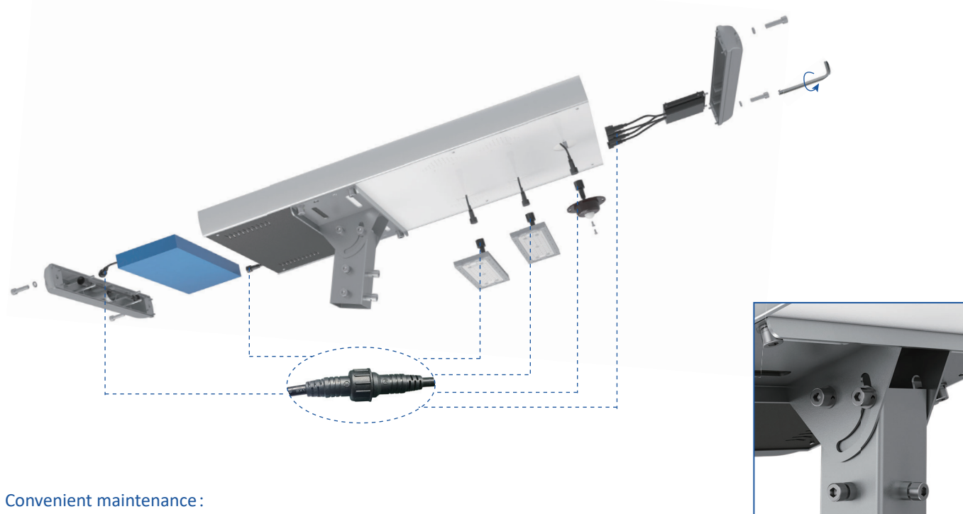
Angle of Mounting bracket: 0-90°
